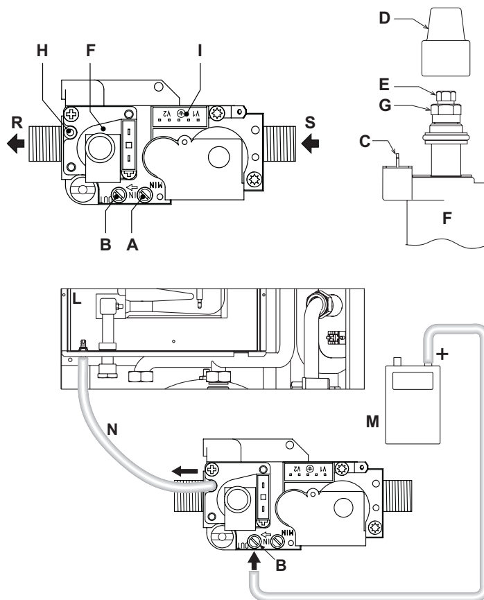
fig. 26 - Valvola gas
